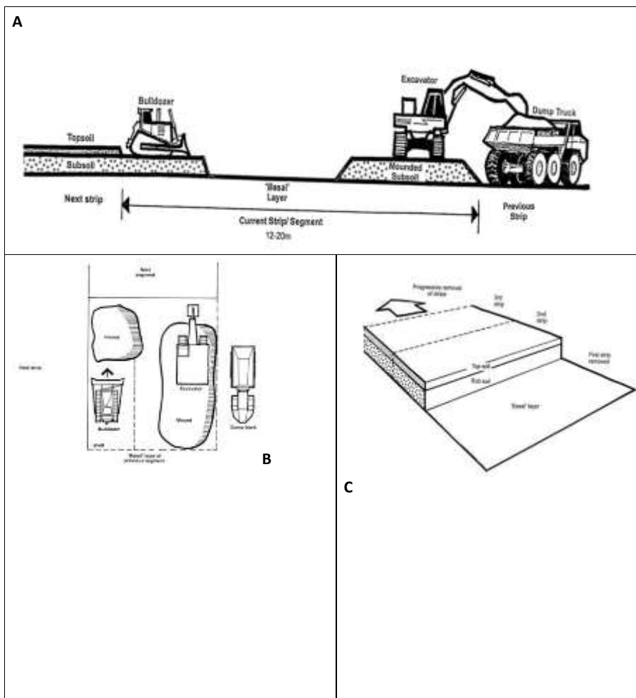
Figure 5.1: Topsoil and subsoil vehicle use (A) stripping with bulldozer, (B) 360° excavator and articulated dump-truck, and (C) the sequential bed stripping method executed with an excavator and dump truck
