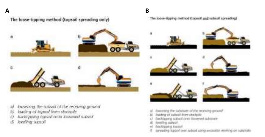
Figure 5.4: The loose-tipping method of soil reinstatement.
